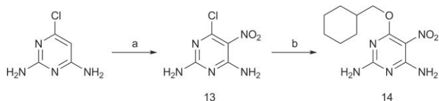
Scheme 3 Reagents and conditions: a) HNO 3 , H 2 SO 4 , 35 °C; b) NaO t Bu, t BuOH, cyclohexylmethanol, 30 °C.
